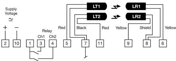
Relay output – MPA 21 A/B 50X
